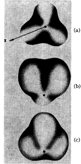
FIG. 4. The simplest possible form of the heavy-hole Fermi surface. The trigonal axis of the trefoloid must be parallel to that of the crystal. The maximum equatorial radii must be parallel to the binary axes of the crystal. (a) View from a direction in the X - Z plane. Trigonal axis shown as a dot. (b) View from a direction in the Y - Z plane. The surface has been rotated 60^\circ about the trigonal axis, relative to (a). Trigonal axis shown as a dot. (c) View along trigonal axis. The arrow depicts a binary axis.
